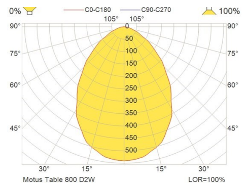
Symmetrical Light Distribution
